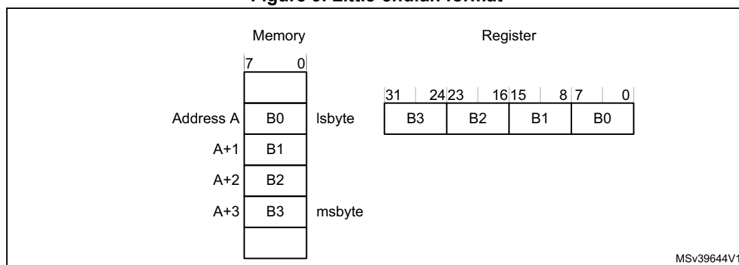
Figure 9. Little-endian format
