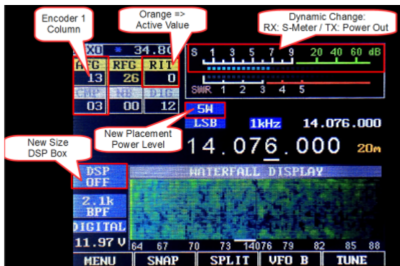
UHSDR Basic Screen Layout (from Github UHSDR)
