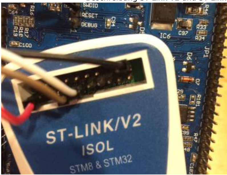
Connection ST-Link to UI board (photo F4HTX)
